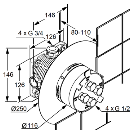
Dimensional drawing
