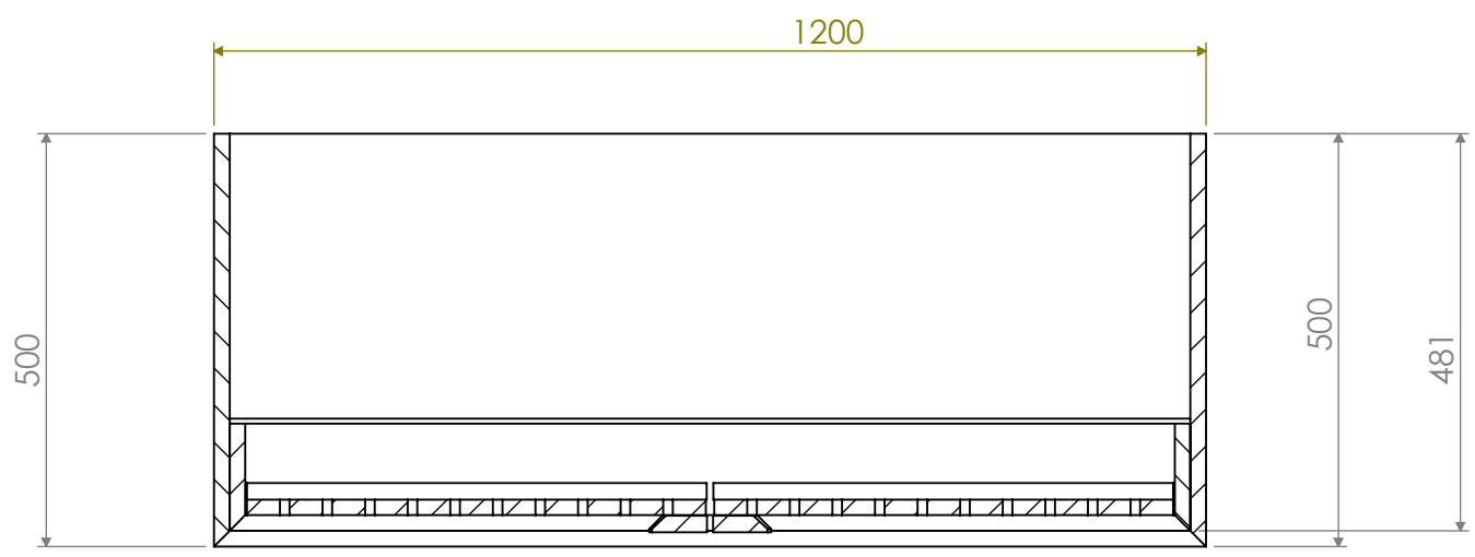
SECTION B-B
